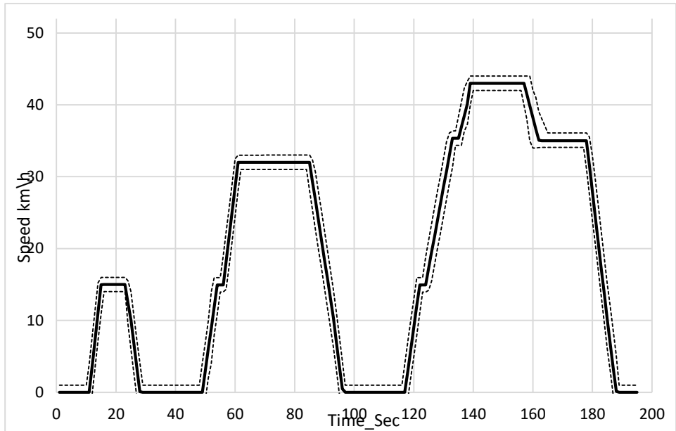
Fig 1 (A): SPEED AND TIME TOLERANCES
