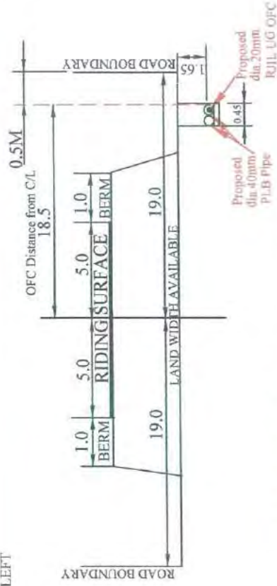
CROSS SECTION @ KM21/100 TO KM21/200
