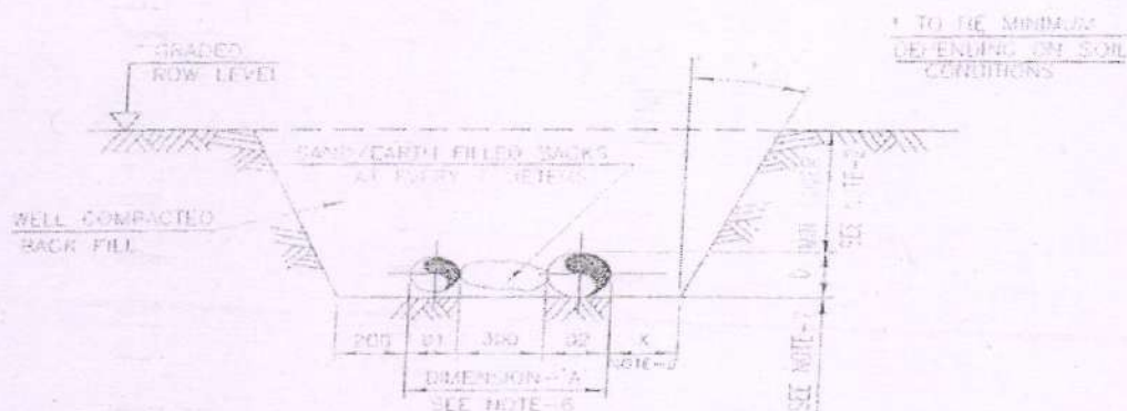
TRENCH IN NORMAL SOIL / CONSOLIDATED ROCK
