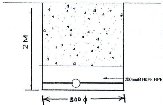
SECTION 1-1 CROSS SECTION ON ALONG ROAD BY HDD METHOD AT SARUA BAGHMARI ROAD [CH. 285/300]
