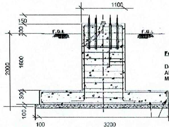
SECTIONAL ELEVATION
